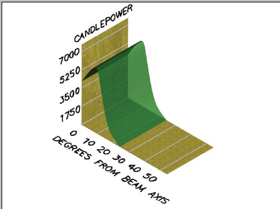
Light output distribution chart
