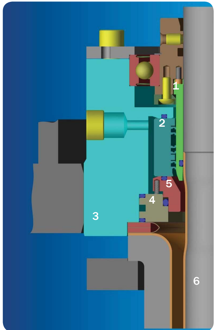
1 Ceramic Sleeve 2 PTFE Sealing Element 3 Stainless Steel Metal Seal 4 Ceramic Adapter 5 Ceramic Balance Piston 6 Agitator Shaft Housing
